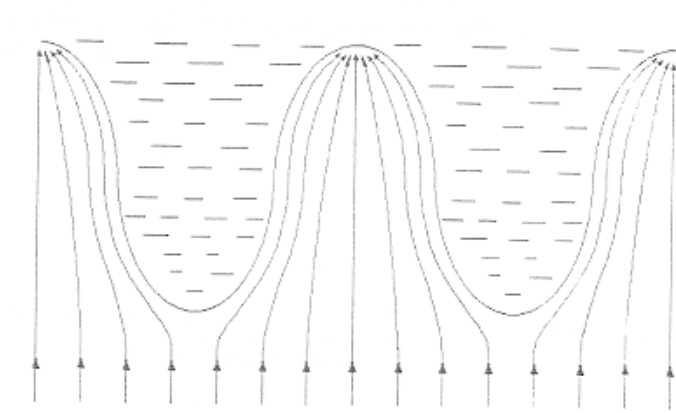
Figure 4. The distribution of the normally oriented magnetic field in the film of the superconducting liquid.
