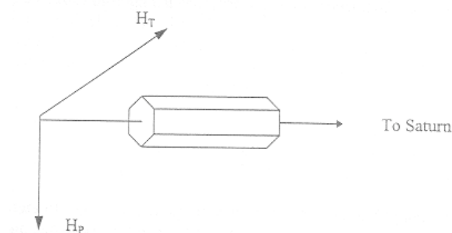
Figure 5. Orientation of the ellipsoidal prism of the superconducting iced particle of the rings in the magnetic field of the Saturn.
